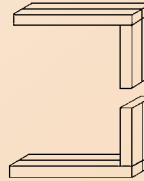
Pouch Pack Seal Assembly Horizontal Seal Below Vertical Seal (For Multiple Loose Items)
